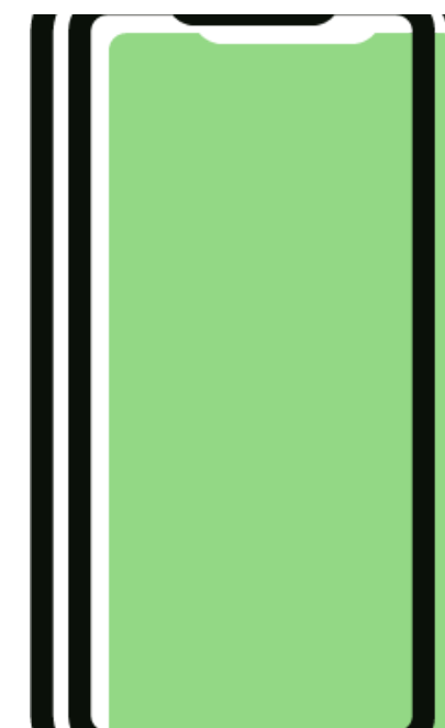
User App
